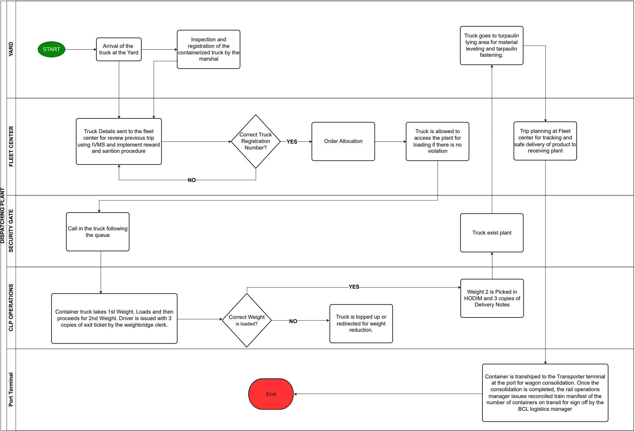
Process Flow for Automated Weigh Bridge-Containerized Clinker Transfer
